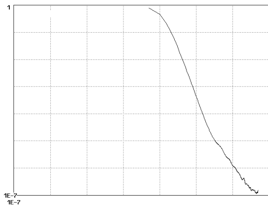
Figure 3. Power spectrum of fluctuations in cluster probability.
