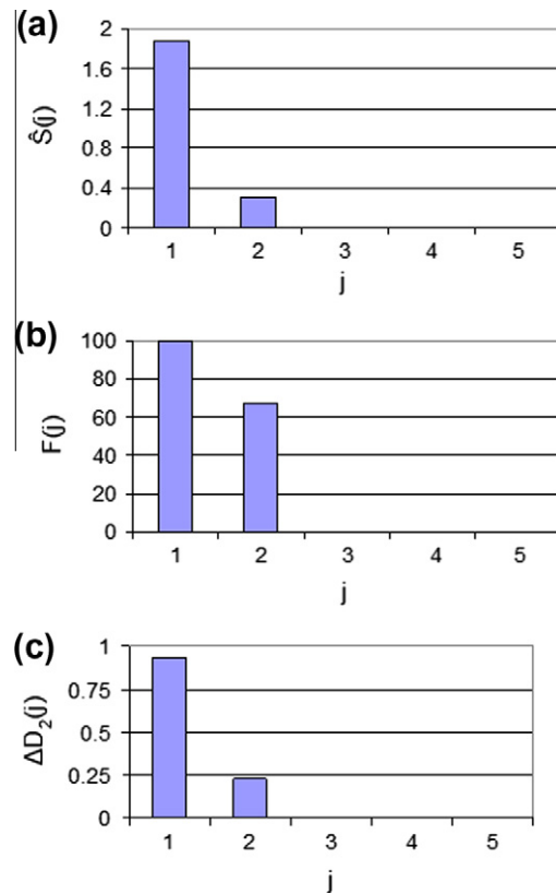
Fig. 3. Embedding calculations for simple Hénon map using (a) neural network sensitivities, (b) false nearest neighbors, (c) correlation dimension.
